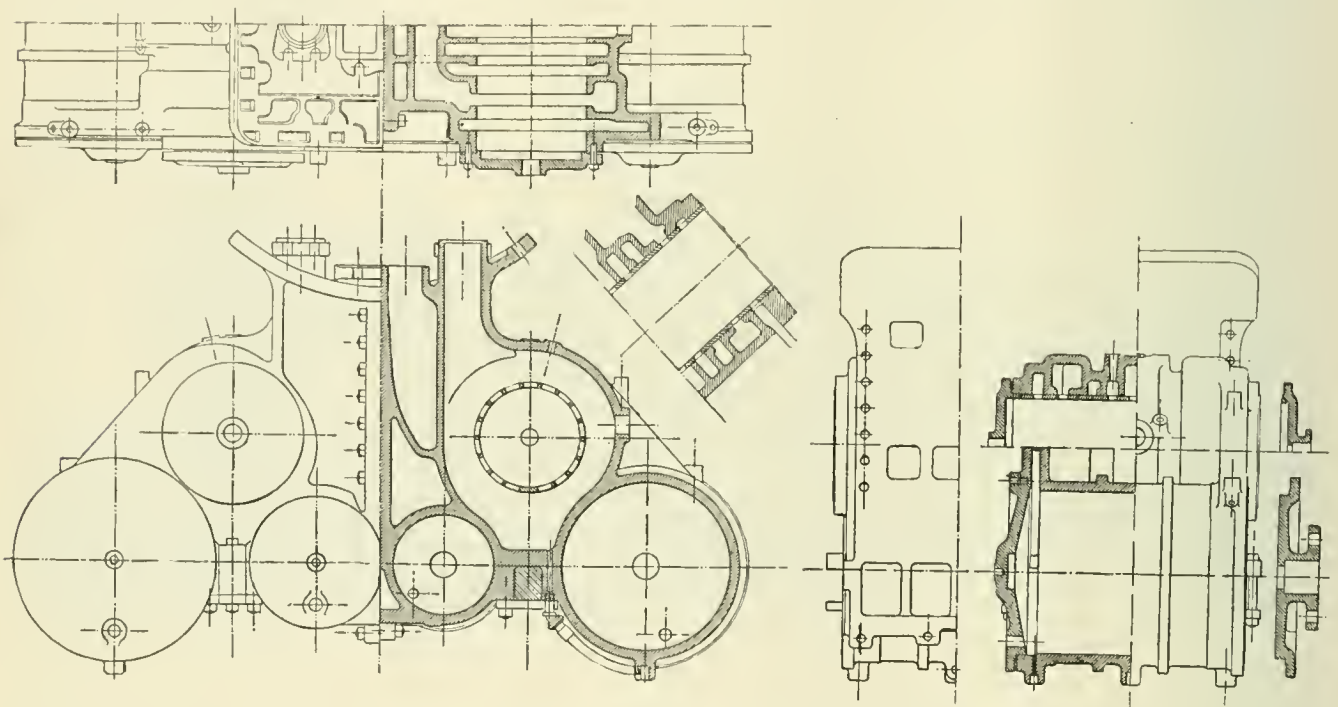
CYLINDER ARRANGEMENT OF VAUCLAINE'S BALANCED COMPOUND.
